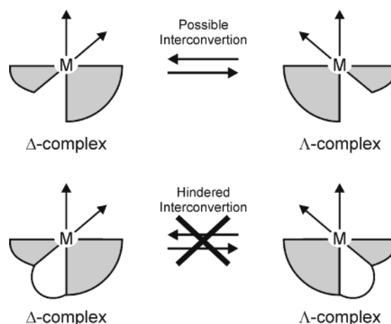
Scheme 9
