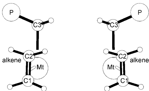
Chiral orientations of a primary growing chain
