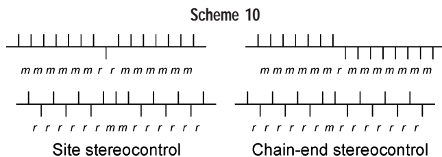
Scheme 11 (-)growing chain (+)growing chain
